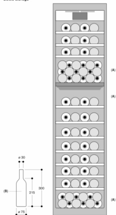
A: Suitable area for storage of magnum bottles in standard tray configuration B: 0.75 liter Measurements in mm
